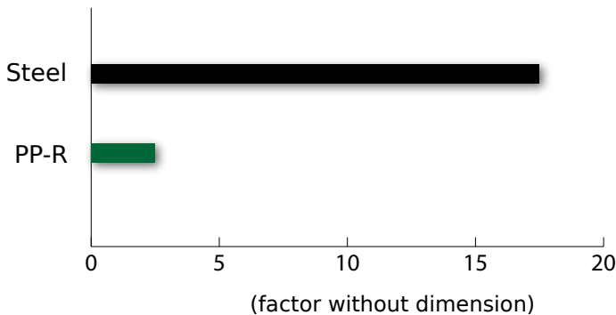
Standardized Comparison (VENOB) of Various Pipe Materials Impact on the Environment - Emissions in Air
