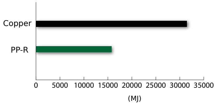
Energy Equivalent Value of the Complete Piping System for a 16-Family Housing Complex
