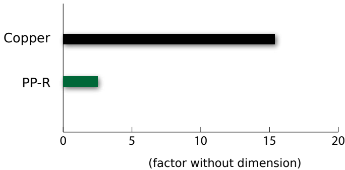
Standardized Comparison (VENOB) of Various Pipe Materials Impact on the Environment - Emissions in Air
